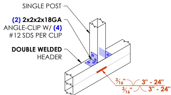
1 ABOVE HEADER DETAIL SCALE: 3/4" : 1'
