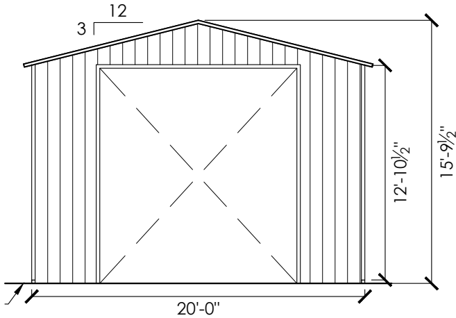
FRONT END WALL ELEVATION SCALE: 1/8" : 1'
