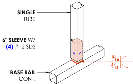
4 COLUMN-BASE DETAIL SCALE: 3/4" : 1'
