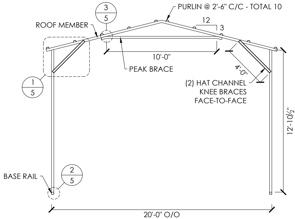
TYPICAL FRAME SCALE: 3/16" : 1'
