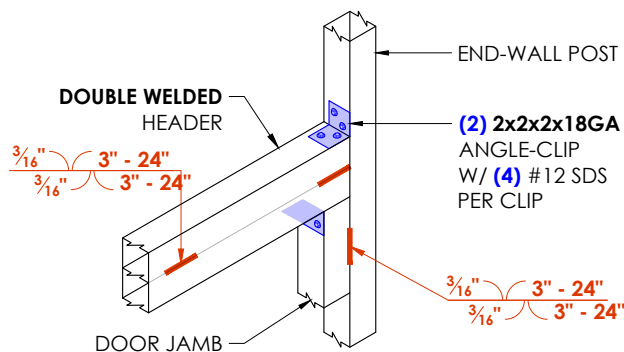
3 DOOR HEADER DETAIL SCALE: 3/4" : 1'
