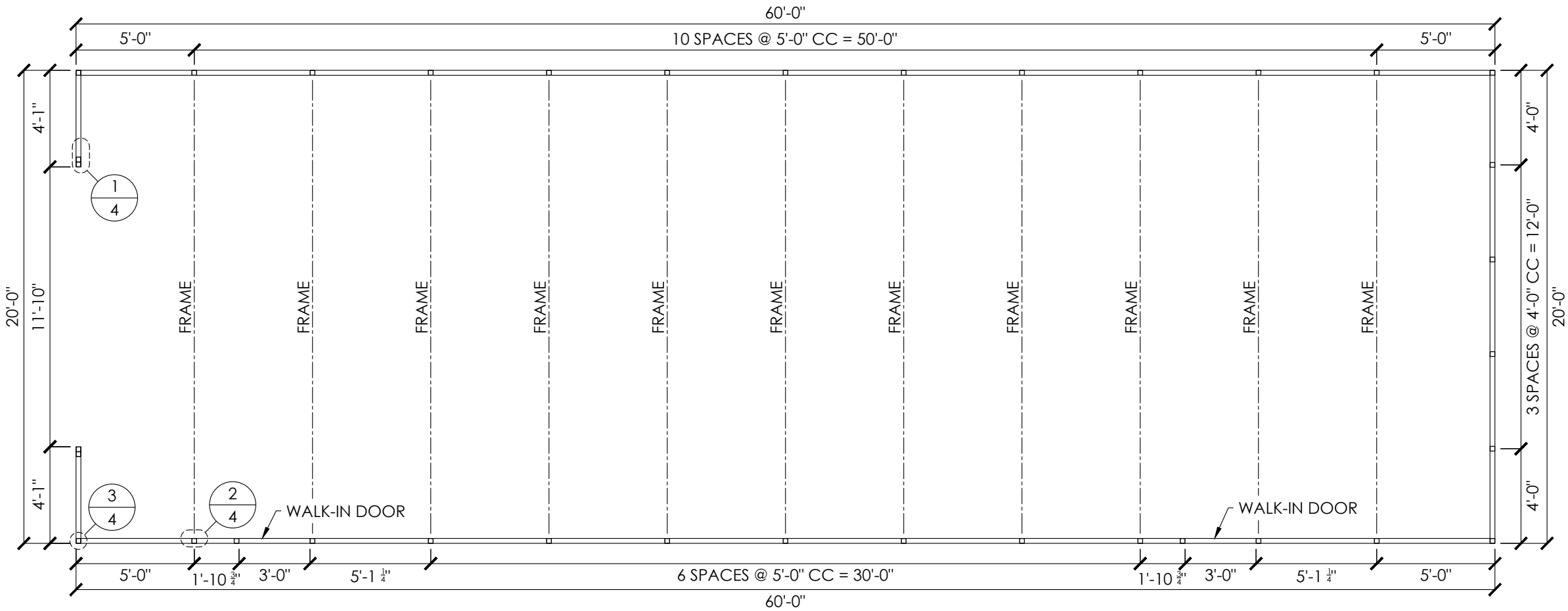
COLUMN LAYOUT PLAN
