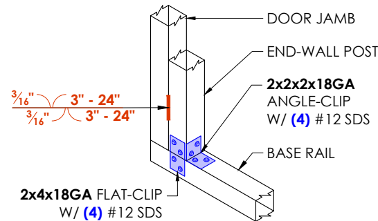
2 DOOR BASE DETAIL SCALE: 3/4" : 1'
