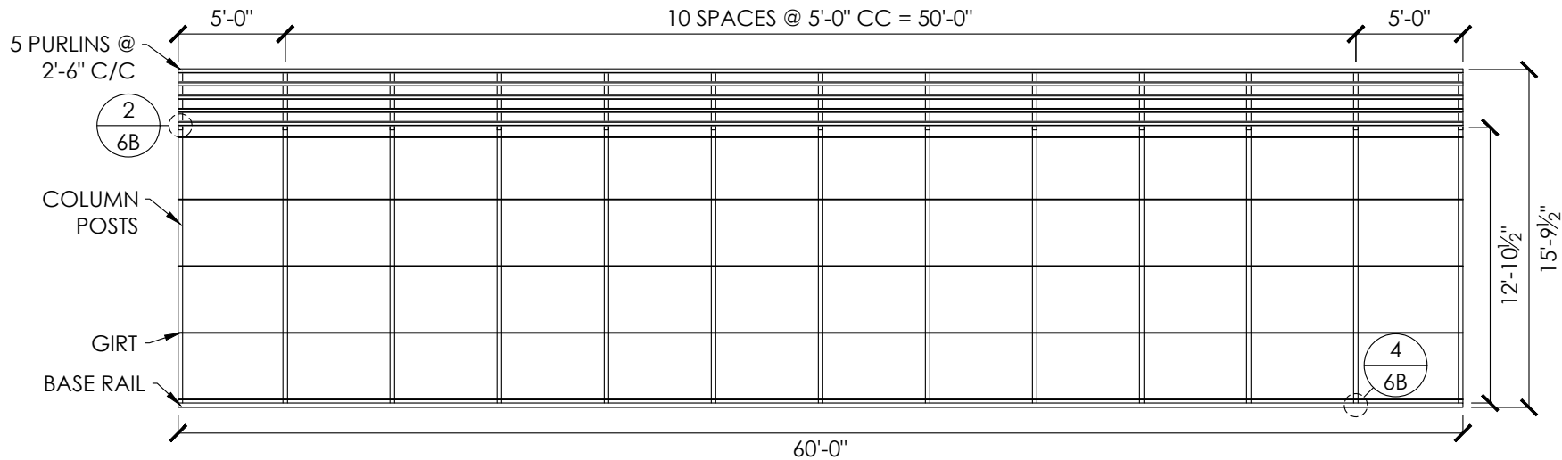
LEFT SIDE WALL FRAMING SCALE: 1/8" : 1'
