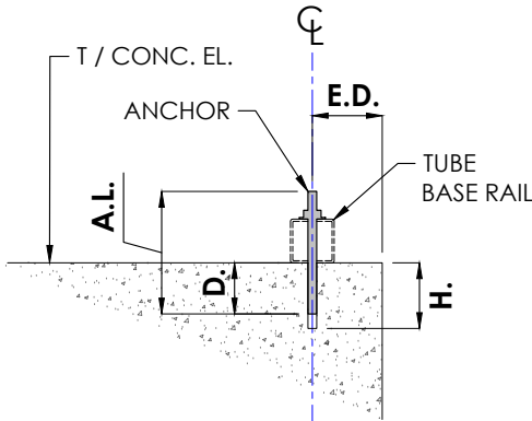
ANCHORAGE DETAIL
