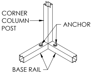
3 ANCHOR DETAIL SCALE: 1/2" : 1'
