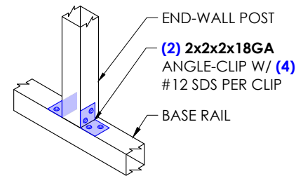
4 COLUMN-BASE DETAIL SCALE: 3/4" : 1'
