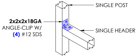
1 WINDOW/DOOR DETAIL SCALE: 3/4" : 1'
