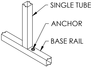
2 ANCHOR DETAIL SCALE: 1/2" : 1'
