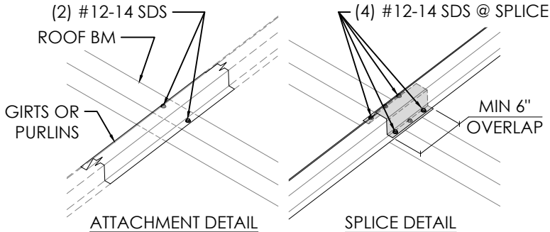
2 GIRT/PURLIN DETAIL SCALE: 3/4" : 1'
