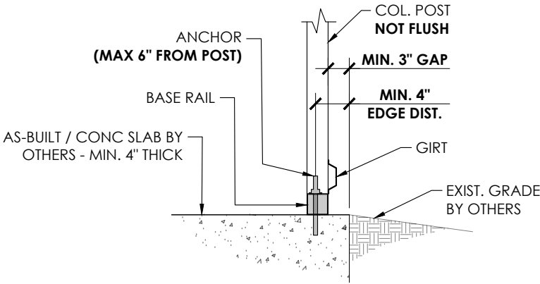
1 ANCHORAGE DETAILS
