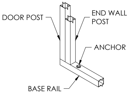
1 ANCHOR DETAIL SCALE: 1/2" : 1'
